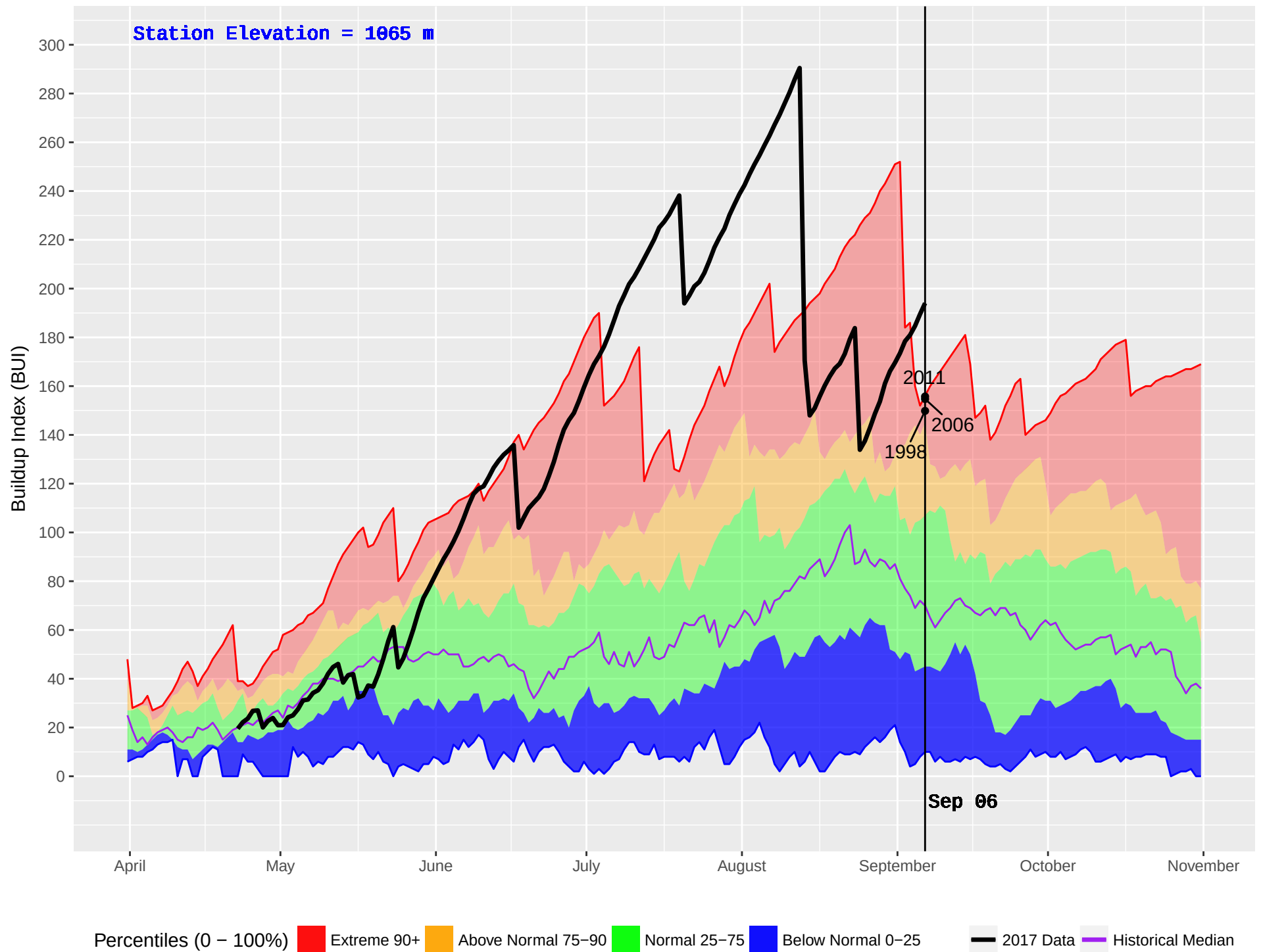
PLACE LAKE (212) : Historical (1981–2016) and Current (2017) Noon Buildup Index (BUI)
